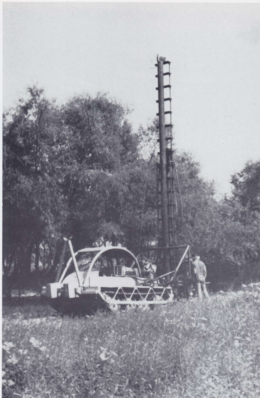
Bombardier vehicle equipped with a boom being used for installing and testing full-size auger anchors (Fig. 2).
