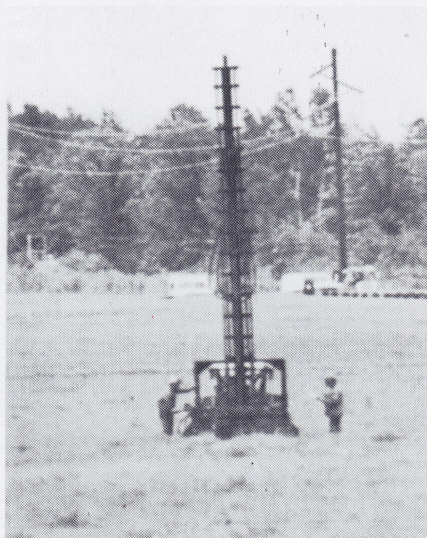
Using pull. After the auger anchor has been inserted into soil to full depth, a pull is made to determine hold down capacity.
