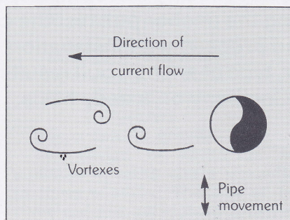
Fig. 3. Vibration caused by vortex shedding in the current flow causes the pipeline to move up and down.
