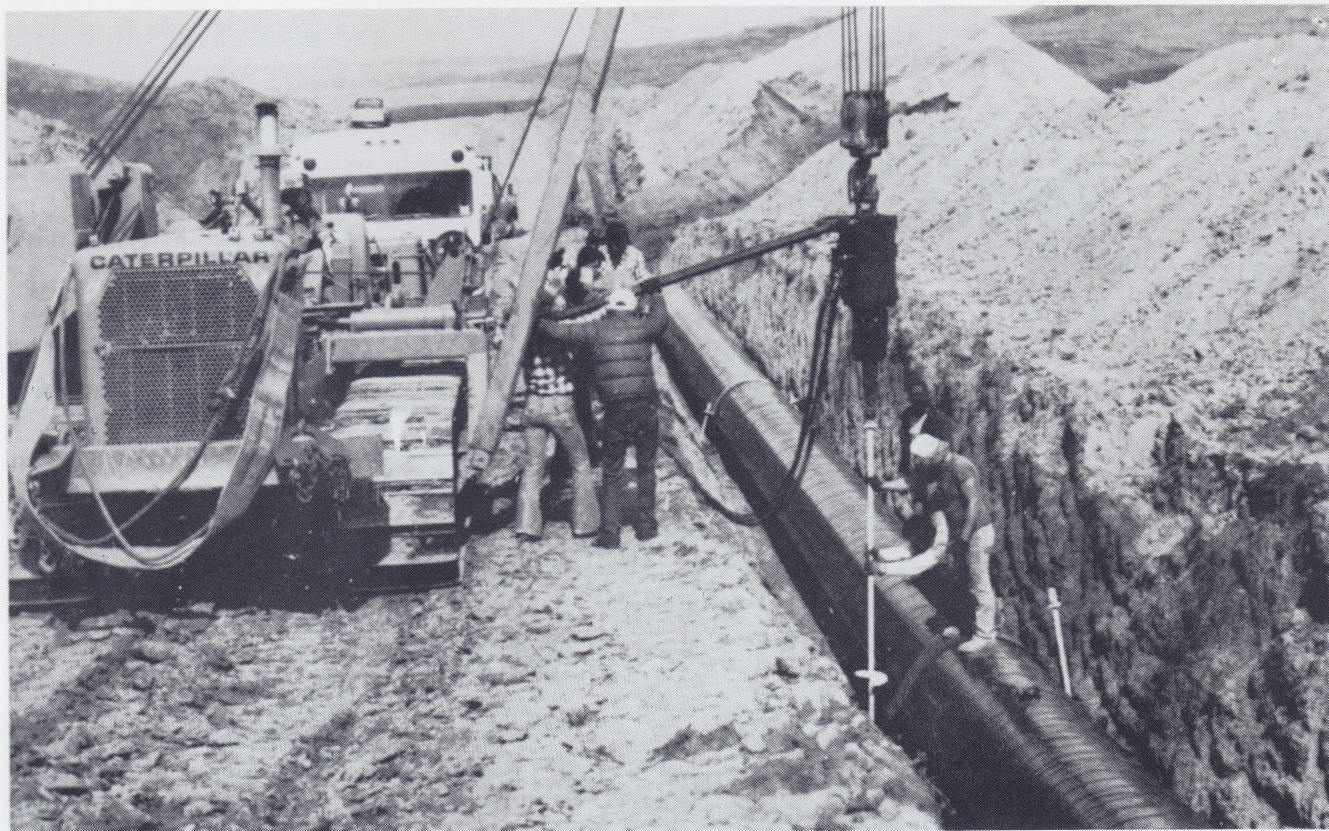
Technique of setting anchors using a sideboom tractor (Fig. 1).
