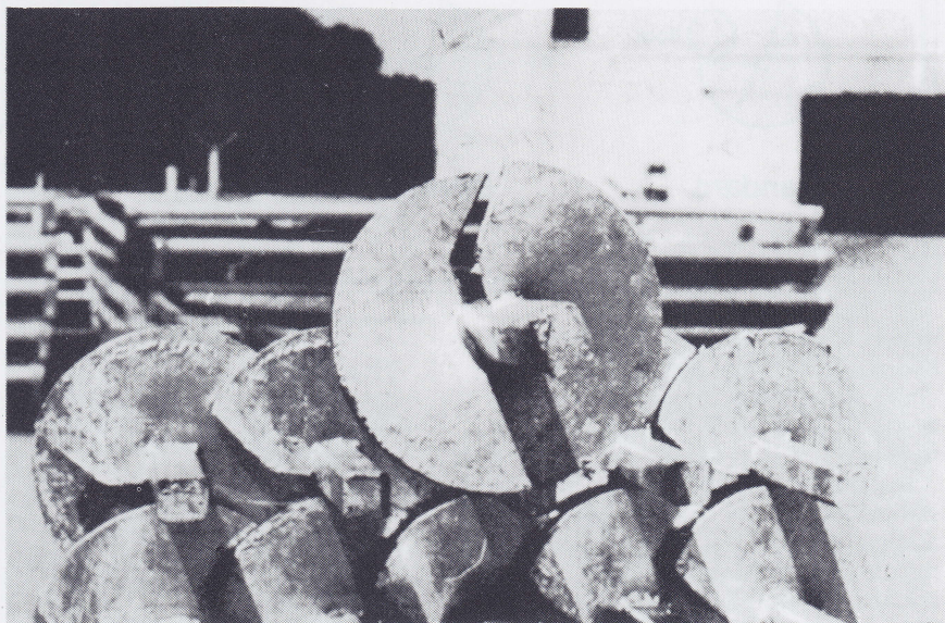
Newly developed beveled fluke on anchors for use in glacial soils (Fig. 5).
