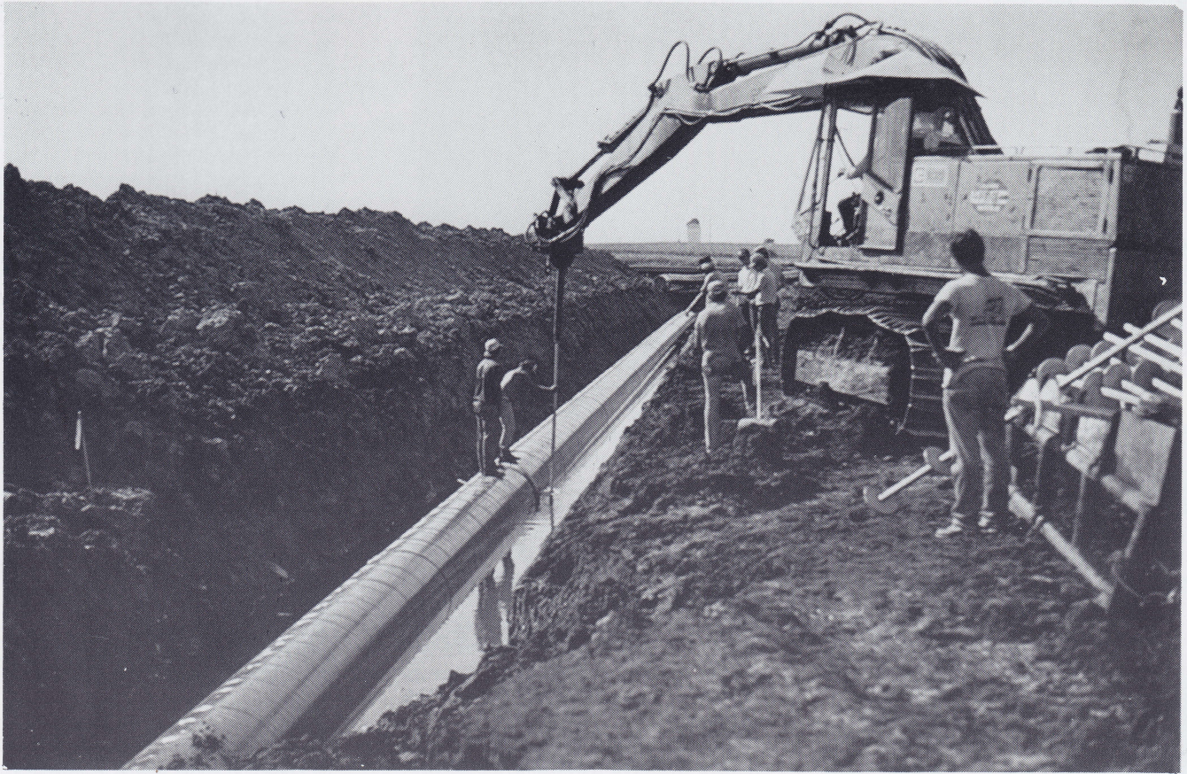
Hydraulic anchor installation tool mounted on backhoe boom turns spiral-type auger anchor into soil; anchors are 10-ft long.
