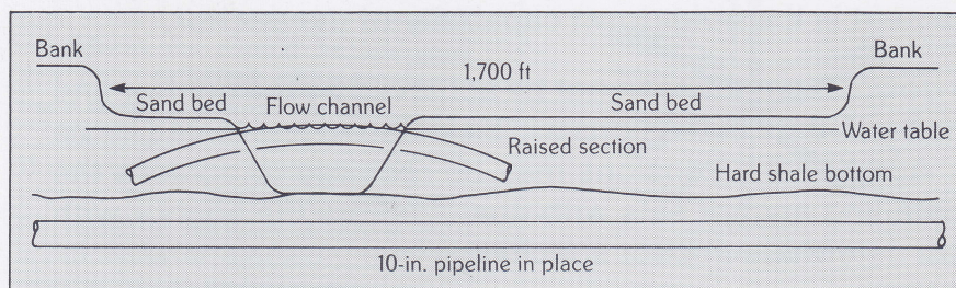
Fig. 1. Crossing stretched 1,700 ft from bank to bank: dotted line shows how pipe moved to water table elevation in the flow channel.
